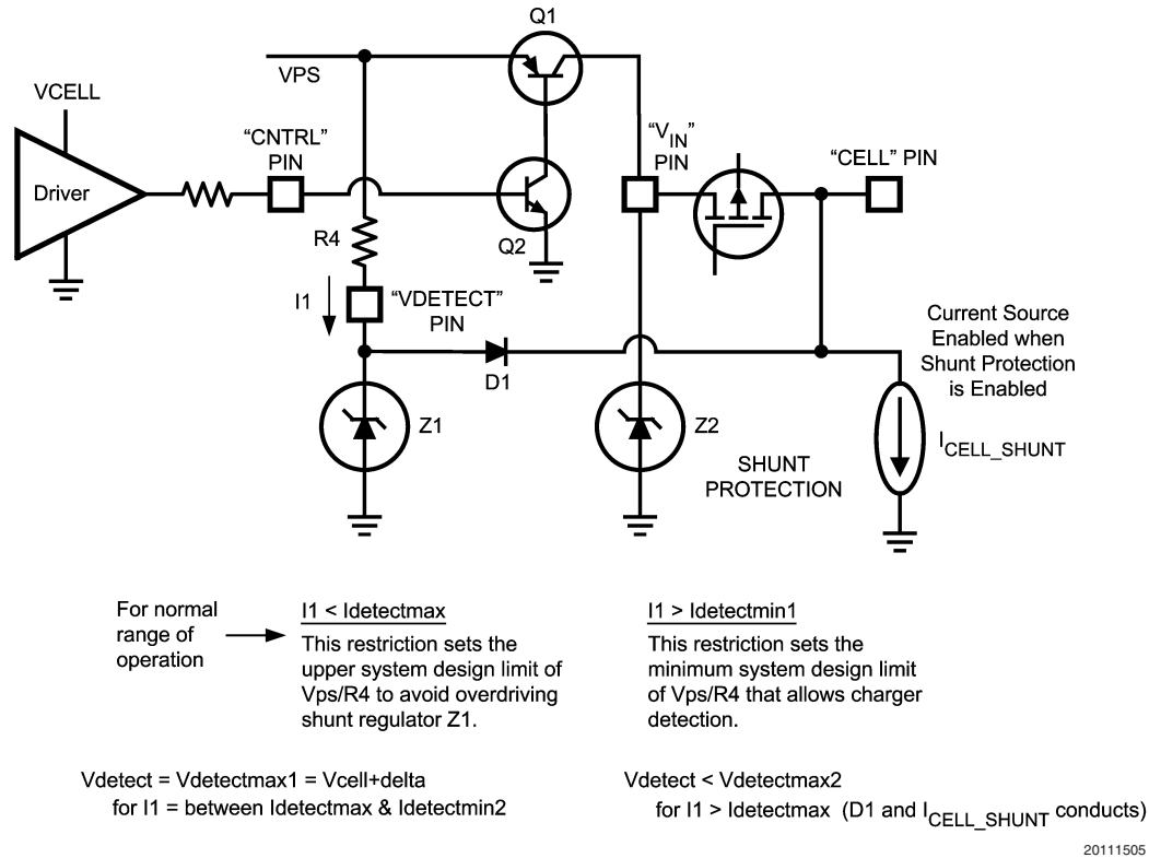
FIGURE 2. V_{\text{DETECT}} Circuit
